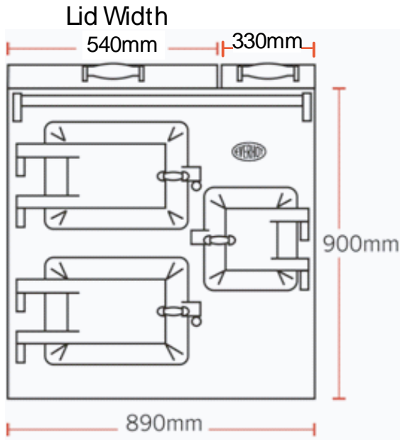
Cooker Width EVH 90i
