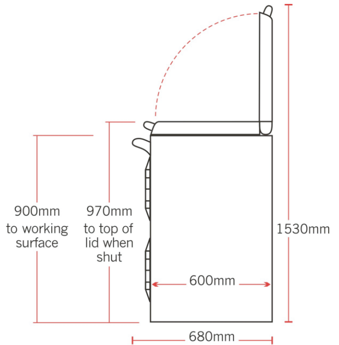
Side View EVH 90i
