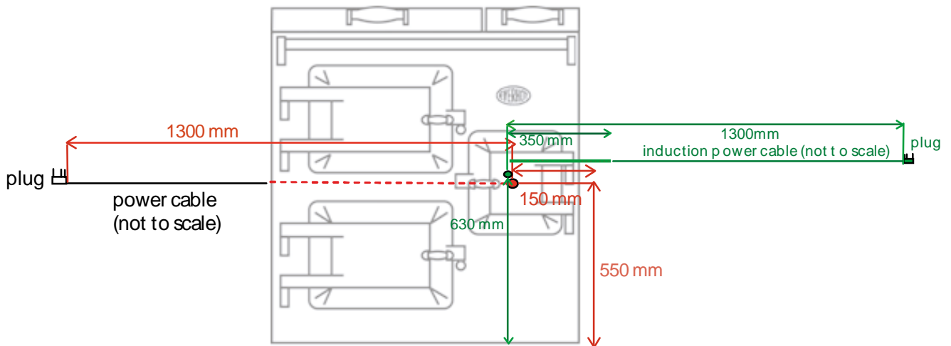
EVH 90i cable lengths
