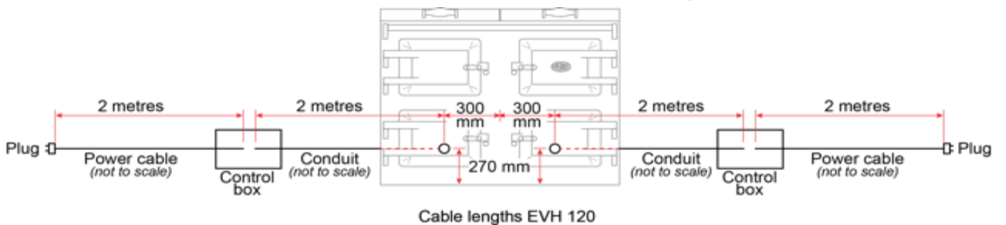
Front view EVH 120
