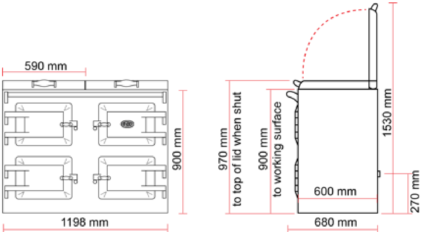
Front view EVH 120
